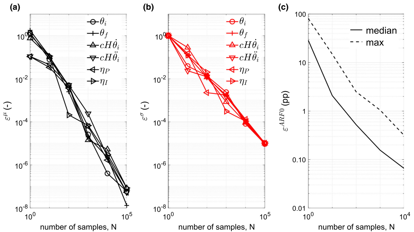
Fig. 4 Dependence of ARFO on Latin Hypercube sample size. Normalized errors in (a) sample mean and b sample variance of input parameters of multiscale model; c median and maximum absolute error in model prediction ARFO (expressed as percentage points, pp) over the validation cohort. For the input parameters, errors are defined with
