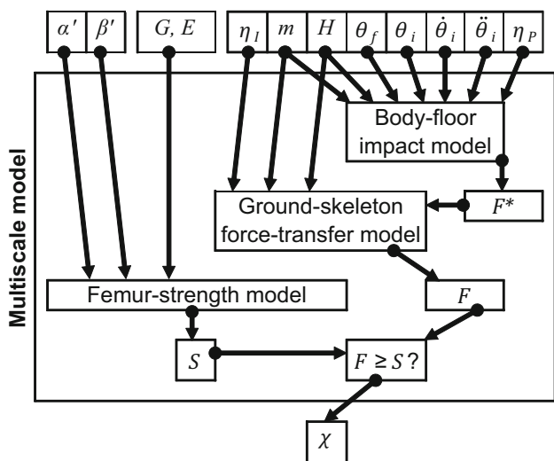
Fig. 3 Orchestration of the multiscale model with input parameters measured at scales from whole body to organ (bone)
