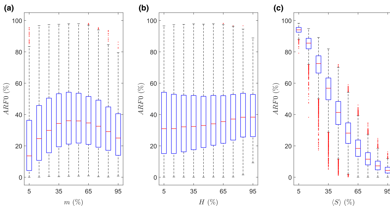
Fig. 5 The variation of ARF0 in a virtual population of 10^5 subjects in dependence of subject-specific parameters: a body mass, m ; b body height, H ; and c bone strength averaged over all orientations, S = \text{mean } S(\alpha', \beta') . Percentage values on the horizontal axes are with (\alpha', \beta')
