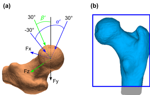
Fig. 2 a In the fall configuration, a concentrated force is applied at the femoral head centre and in a direction specified by the angles \alpha' and \beta' measured with respect to the femoral axes Fz and Fx , respectively. b The surface shown in blue is the region of interest (ROI) where the strain-based fracture criteria are evaluated. The surface outside the ROI, in grey, contains nodes where the solution is judged to be affected either by contact interaction (on the right) or by boundary constraints (at the bottom)
