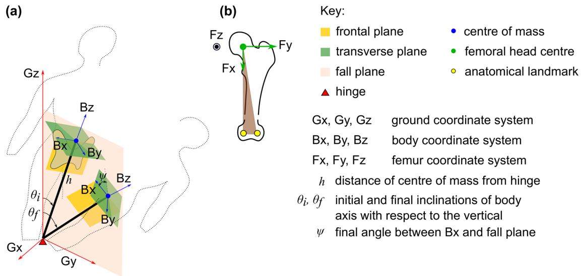
Fig. 1 a The inverted pendulum abstraction of the body during a fall. Coordinate systems for the ground and the body are shown in red and blue arrows, respectively. The origins of the ground and body coordinate systems are identified with the hinge and the body centre of mass,
